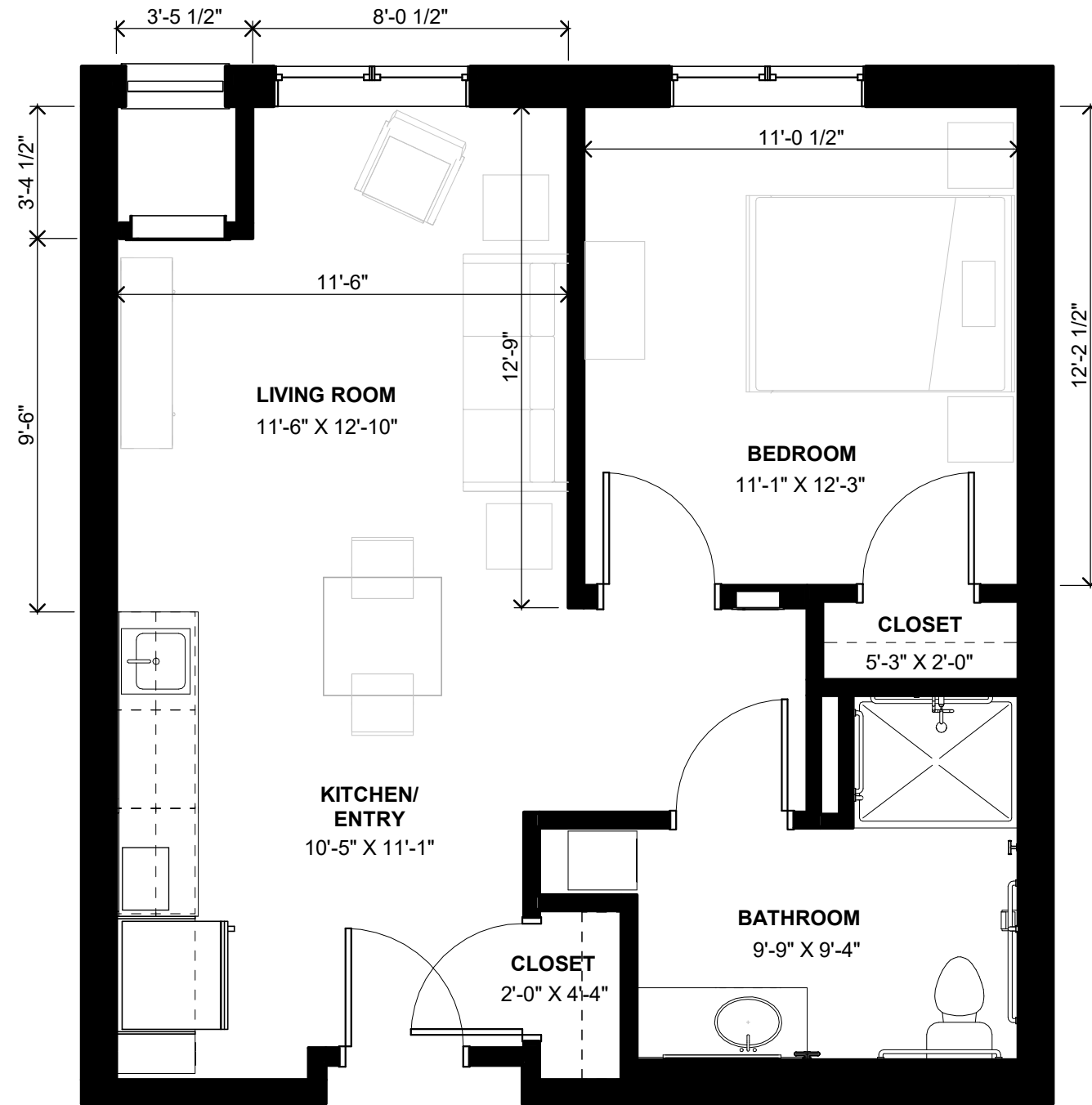
1 UNIT MC3- FLOOR PLAN 1/4" = 1'-0" 0 3' 6'
