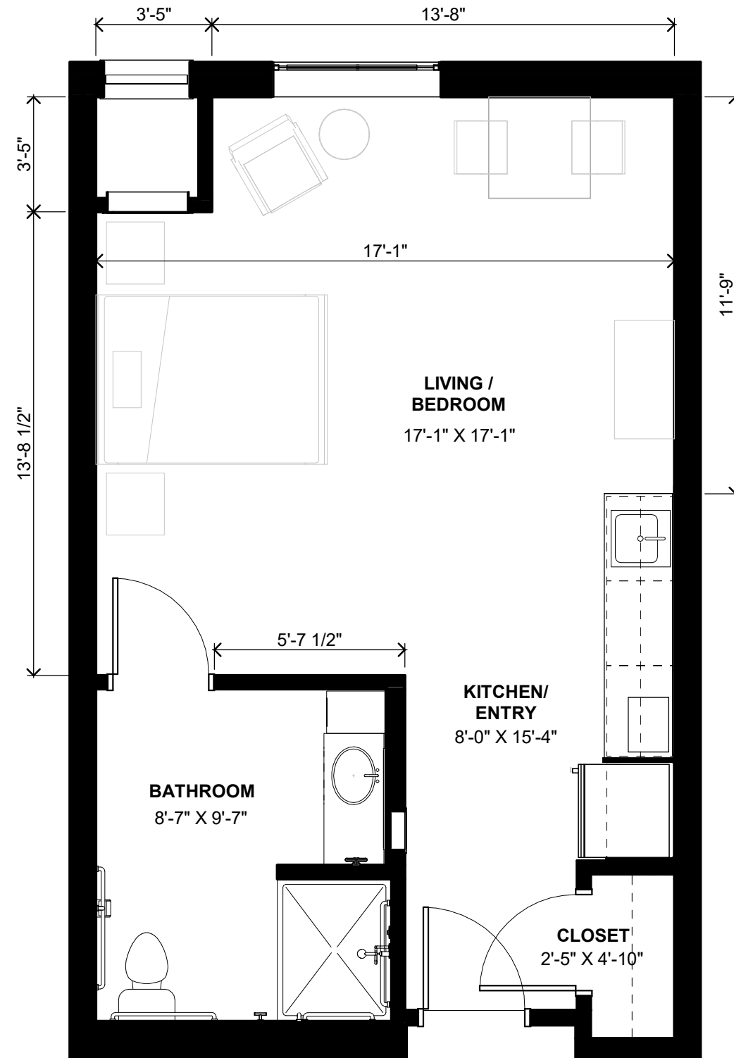
1 UNIT MC2 - FLOOR PLAN 1/4" = 1'-0"
