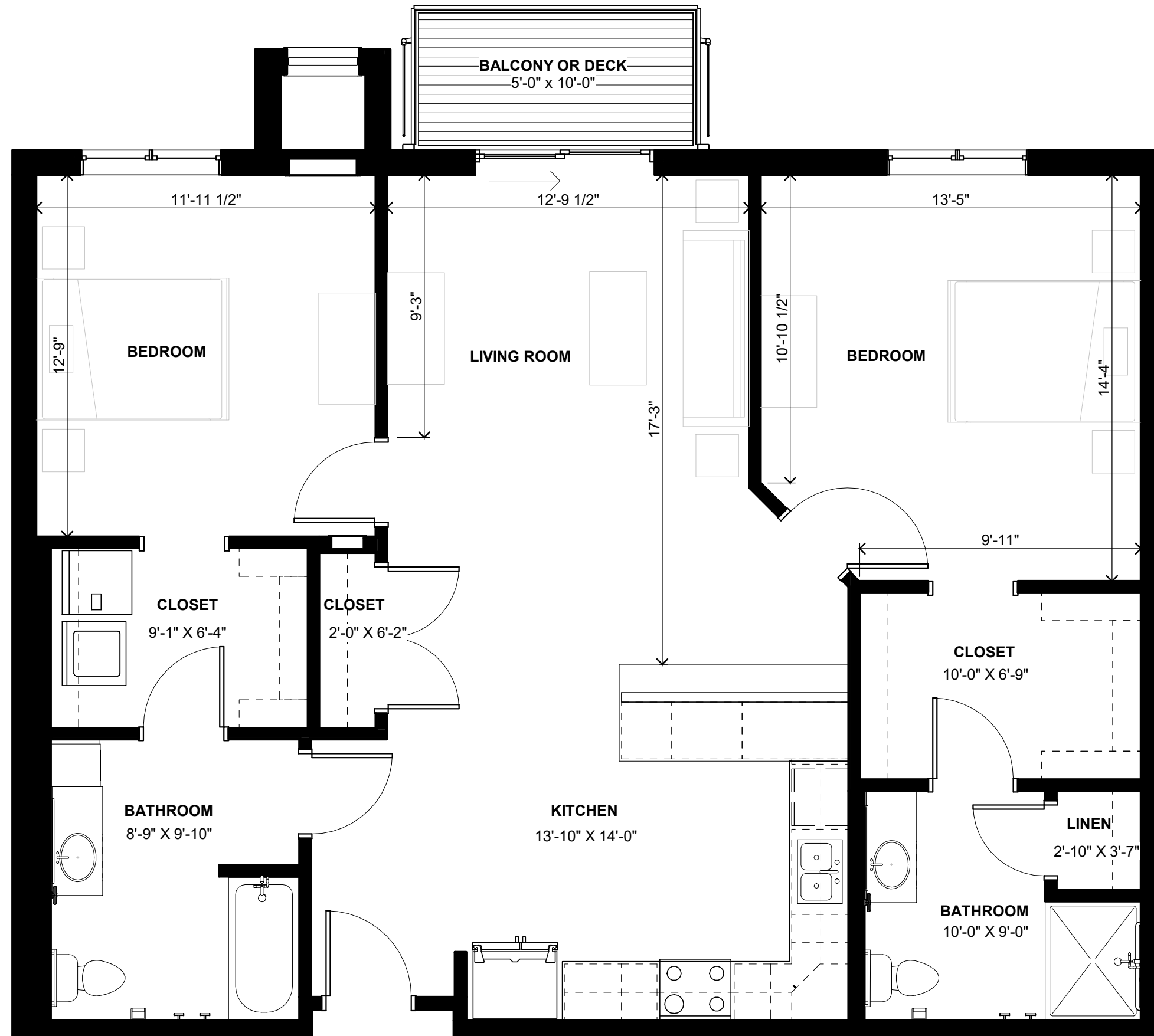
1 UNIT C1 - FLOOR PLAN 1/4" = 1'-0" 0 3' 6'
